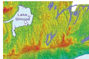
Moraine Groundwater
